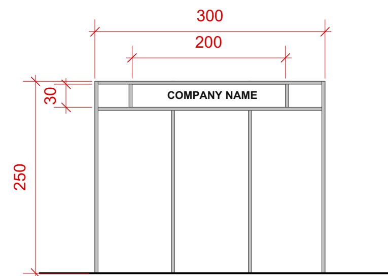
FRONTAL VIEW scale 1:50
